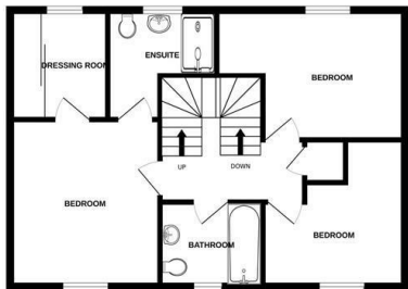
1ST FLOOR 592 sq.ft. (55.0 sq.m.) approx.
